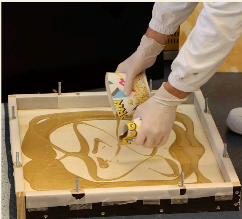
Figure 6: Pouring of the polyurethane foam mixture on top of the plywood
